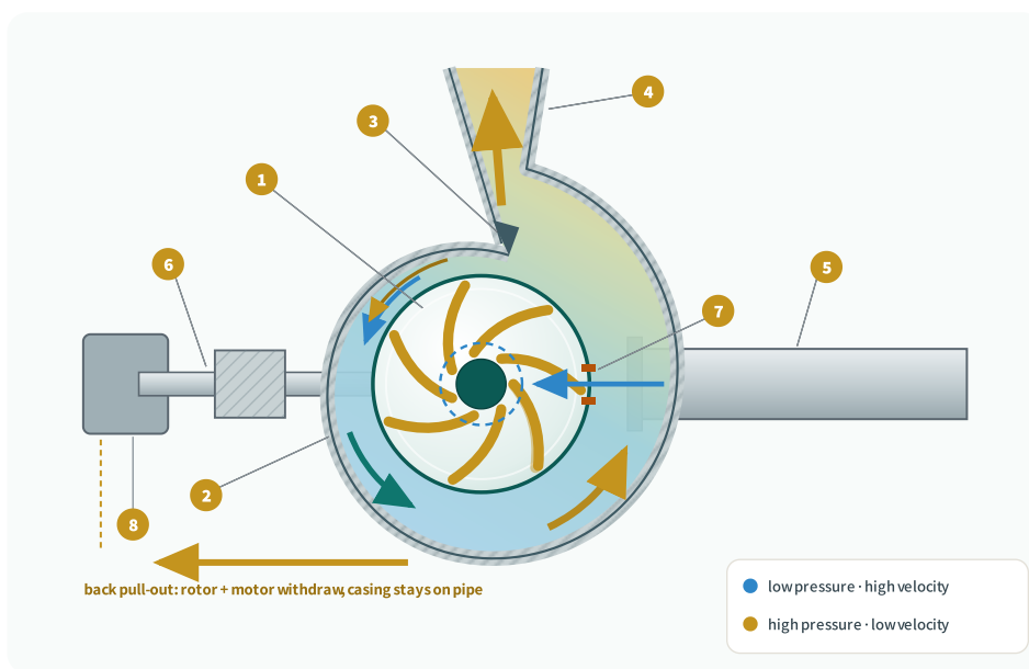
1 impeller · 2 volute casing · 3 cutwater · 4 discharge nozzle 5 suction inlet (axial) · 6 shaft & bearing · 7 wear ring · 8 drive end
