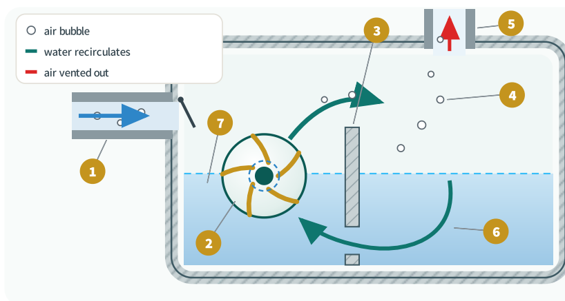
1 suction (air + water) · 2 impeller · 3 baffle & top passage · 4 separation chamber 5 air out via discharge · 6 water returns through port · 7 retained priming water
