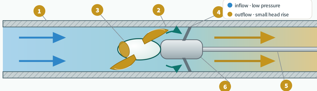
1 tubular casing · 2 twisted propeller blade · 3 hub · 4 outlet guide vanes 5 drive shaft · 6 vane-bearing fairing · flow passes straight through
