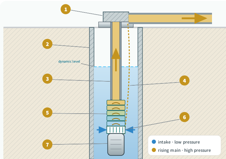
1 wellhead · 2 well casing · 3 rising main · 4 power cable 5 stacked stages · 6 intake screen · 7 submerged motor (water-cooled)
